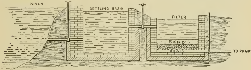
SAND FILTER BED.
